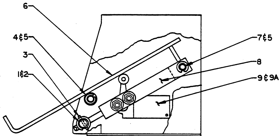
FOOT PEDAL ASS'Y. ~ EARLY MODEL
